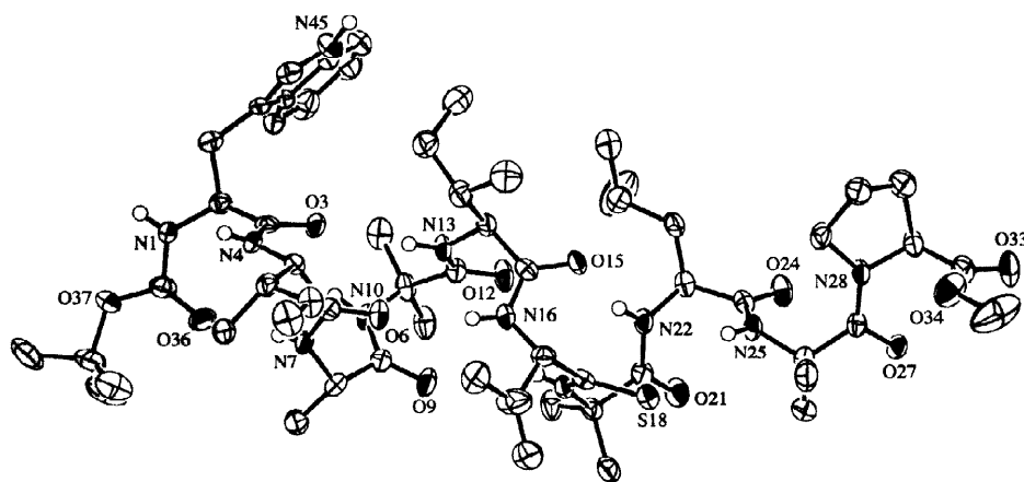
Fig. 1. ORTEP Plot 34 with 50% probability ellipsoids of the molecular structure of BOC-Trp-Ile-Ala-Aib-Ile-ValΨ[CSNH]Aib-Leu-Aib-Pro-OMe ( 12 ) (H-atoms omitted for clarity with the exception of NH atoms)
