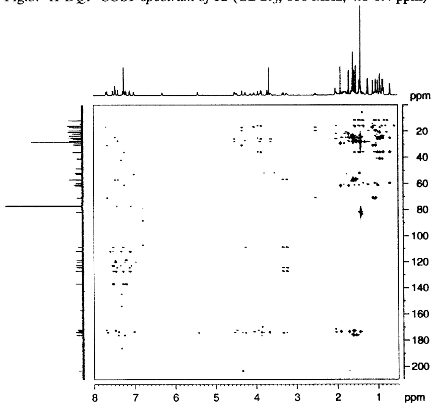
Fig. 4. ^{13}\text{C} , ^1\text{H} -(HMBC) long range-spectrum of 12 ( \text{CDCl}_3 , 600 MHz; 8.0–0.5 ppm and 210–0.0 ppm, respectively)
