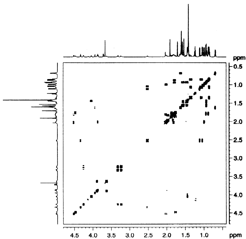
Fig. 3. ^1\text{H} -DQF-COSY-spectrum of 12 ( \text{CDCl}_3 , 600 MHz; 4.8–0.4 ppm)
