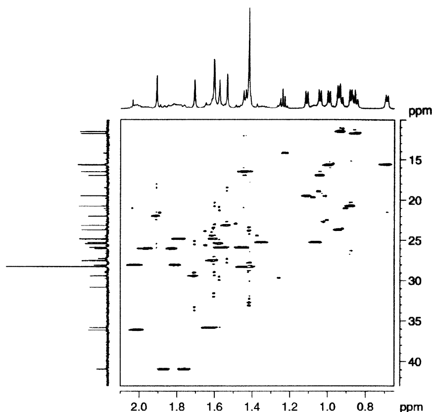
Fig. 5. ^{13}\text{C} , ^1\text{H} -HSQC-spectrum of 12 ( \text{CDCl}_3 , 600 MHz; 2.5–0.5 and 43–10 ppm, respectively)
