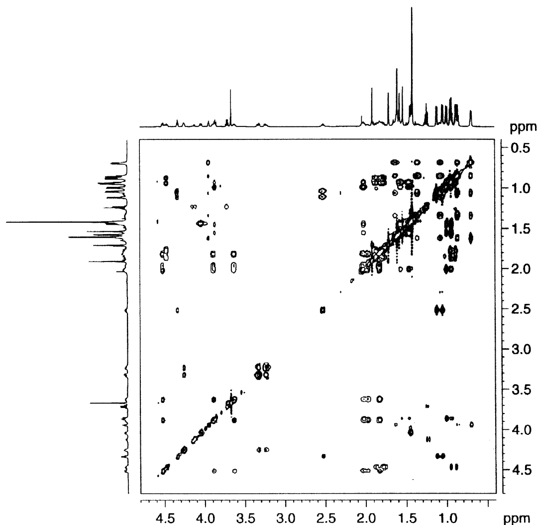
Fig. 2. 1 H-TOCSY-spectrum of 12 (CDCl 3 , 600 MHz; 4.8–0.4 ppm)
